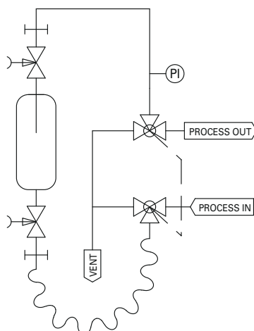
outage tube configuration (F3)
